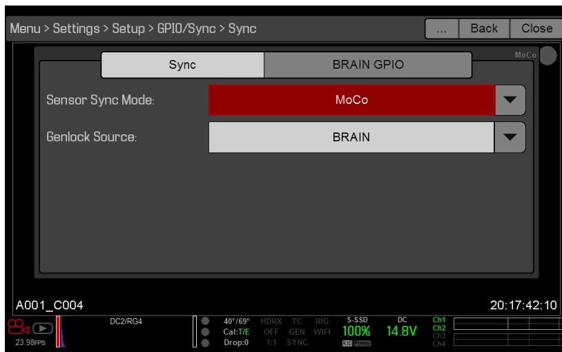
Figure: MoCo Sync Settings
