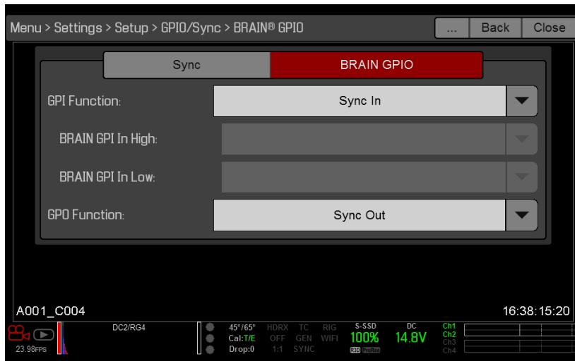
Figure: MoCo BRAIN GPIO Settings
